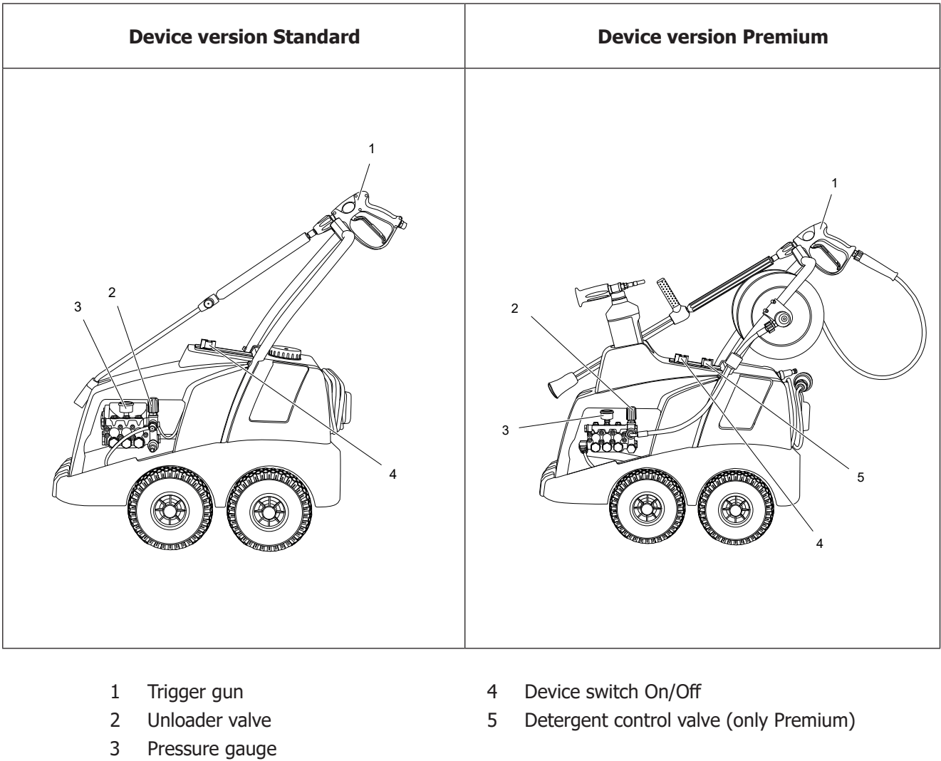
Fig. 6 - 1 Controls and indicator elements, examples for version Standard and Premium
