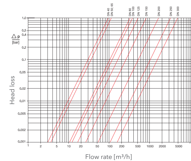
Typical Head Loss Curve
