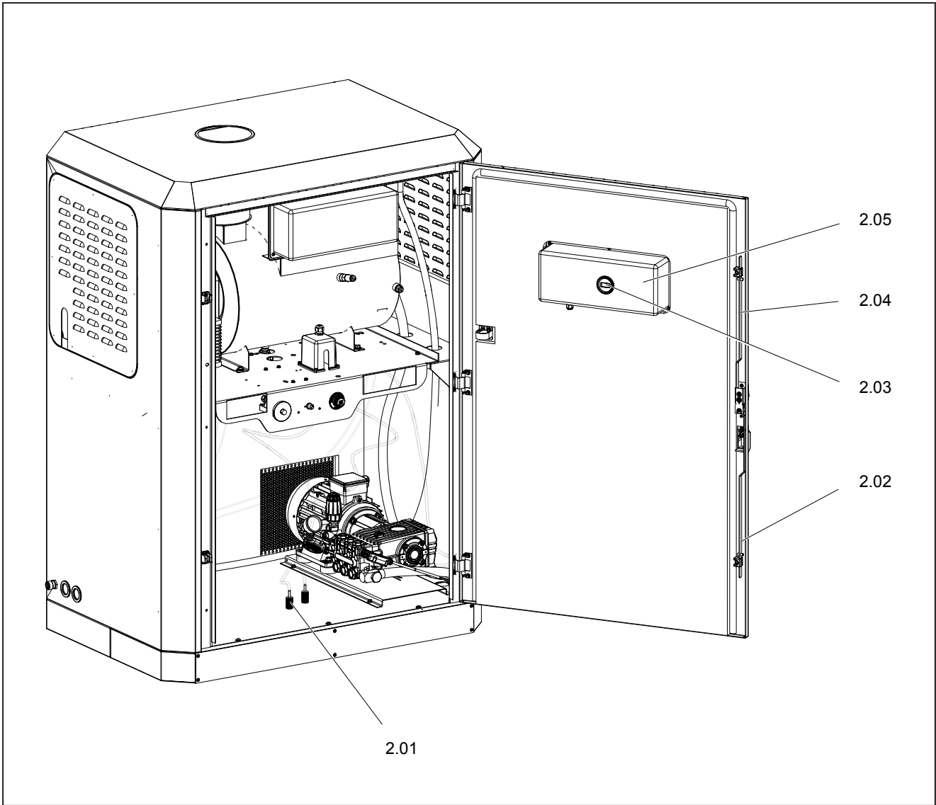
Fig. 10 - 2 System cabinet (interior)
