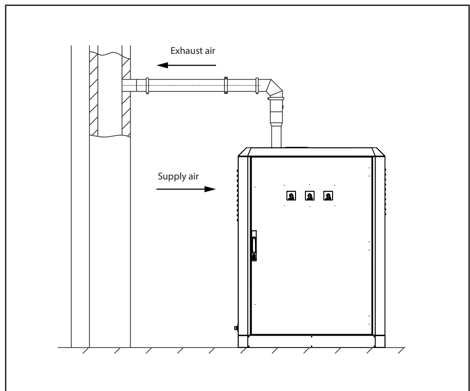
Fig. 4 - 2 Installation location within buildings (example for installation location independent of room air)
