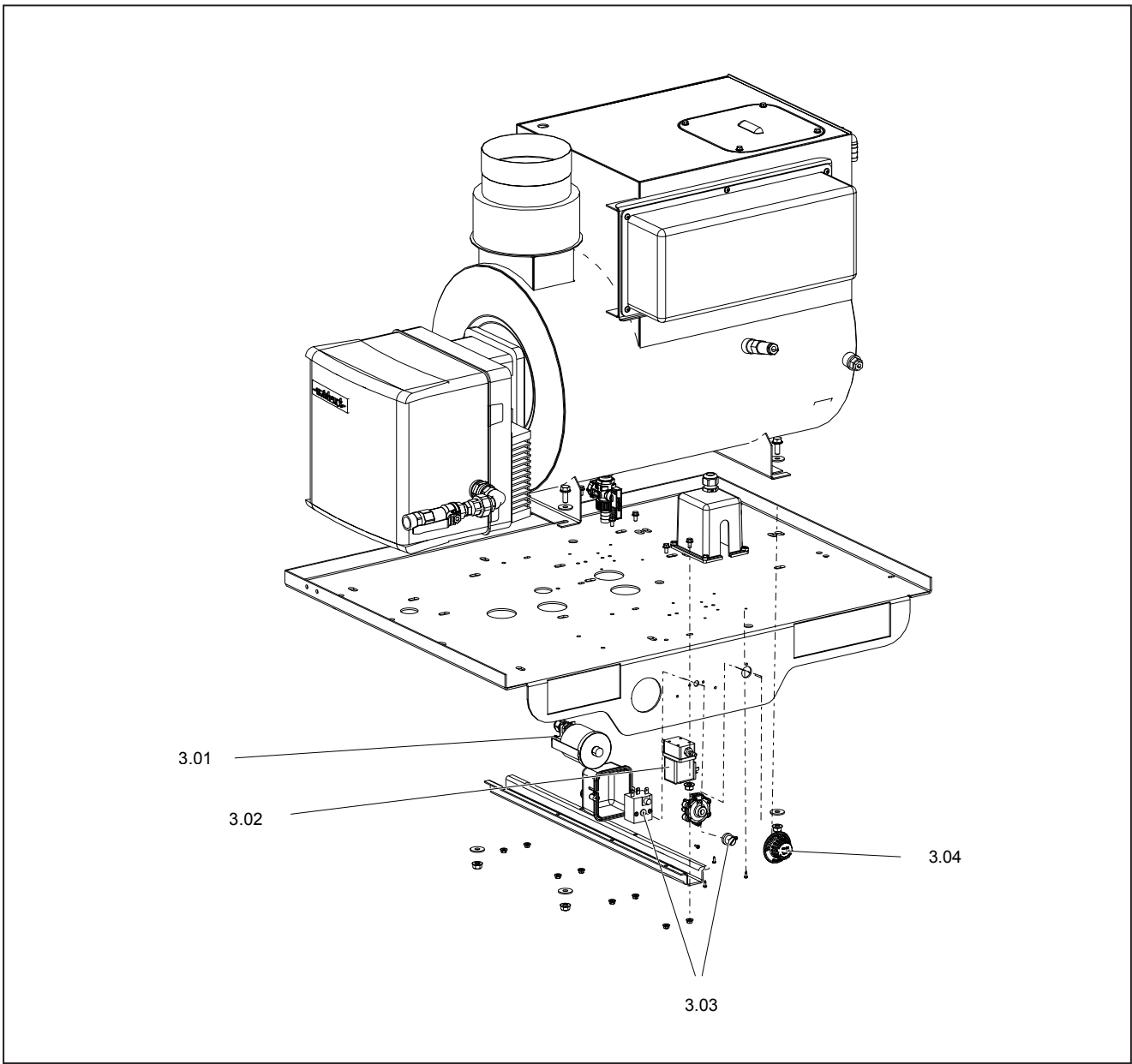
Fig. 10 - 3 Components on chassis middle section, exploded view
