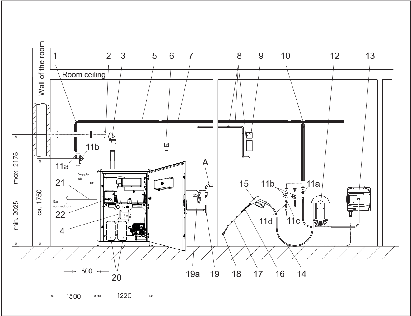
Fig. 4 - 3 Installation material for installation site inside buildings, general example
