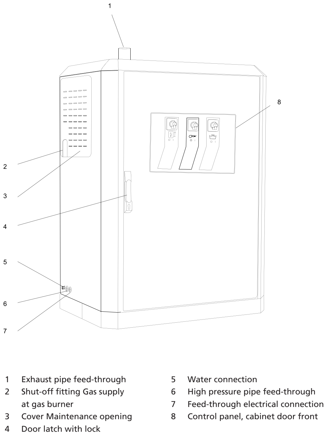
Fig. 3 - 1 High Pressure Cleaner, Hot Water, Stationary, HSC1140-INOX Gas, total view
