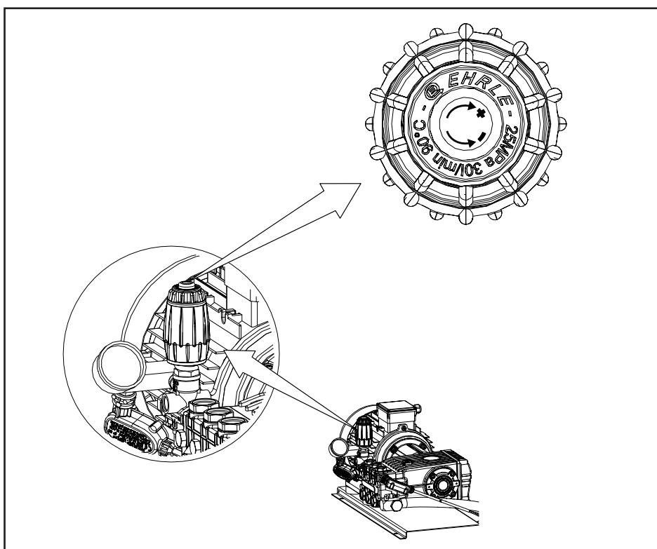
Fig. 6 - 4 Adjustment of the operating pressure at the unloader valve
