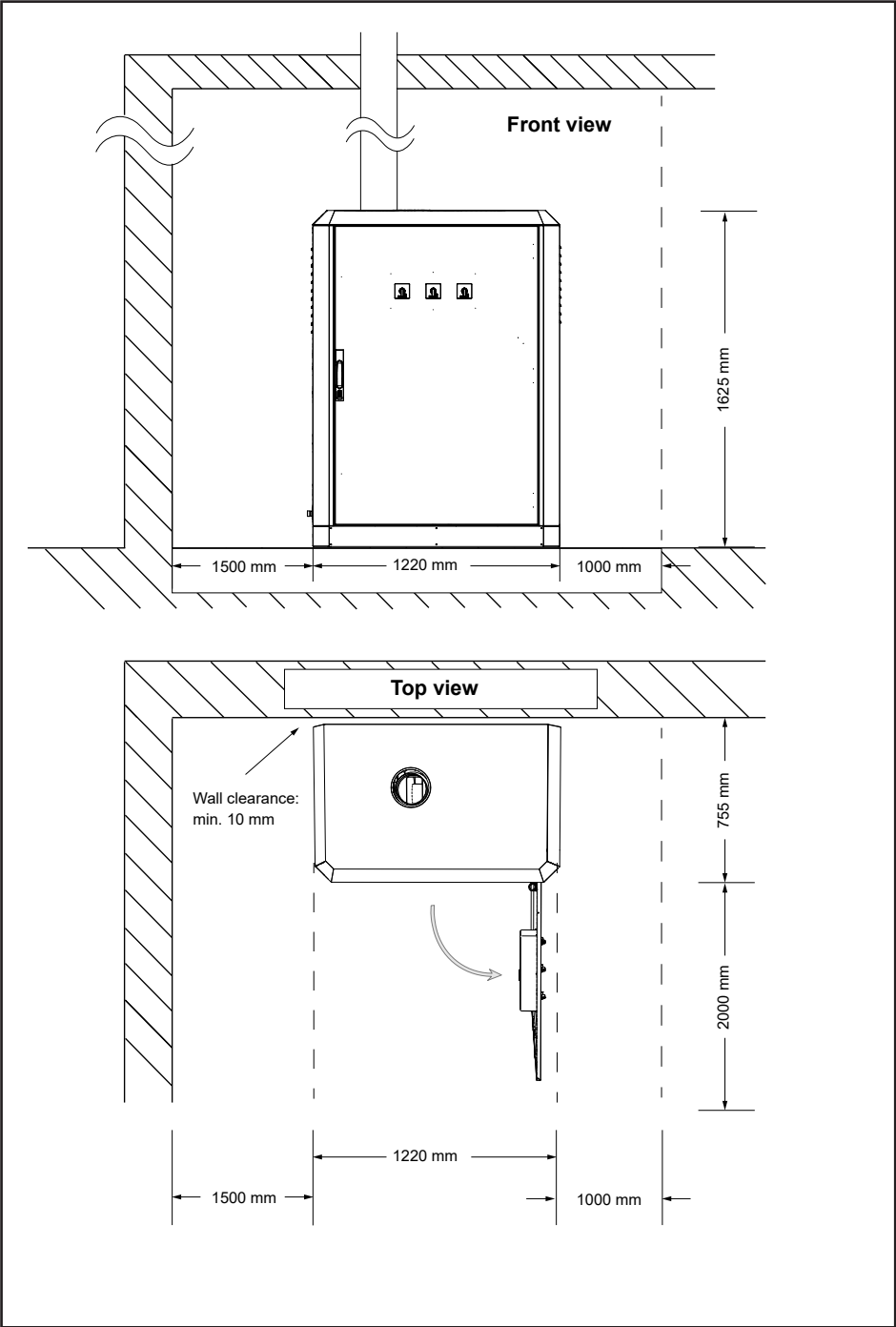
Fig. 4 - 1 Required dimensions for system operating location
