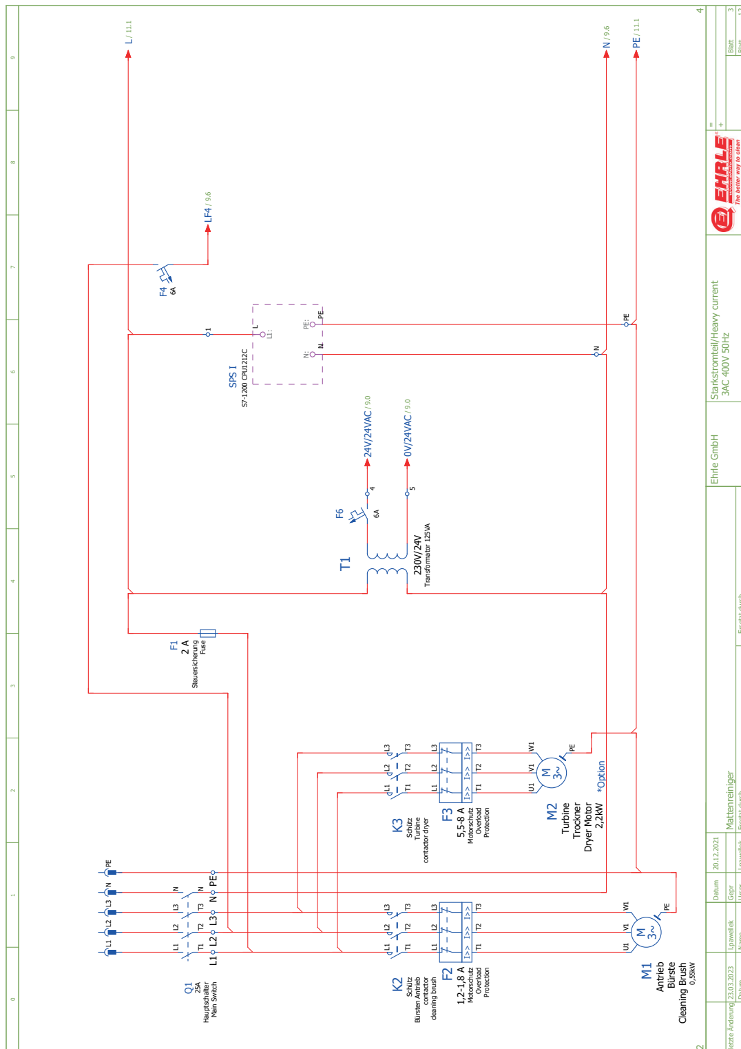
Fig. 11 - 3 Heavy current 3 x 400 VAC, circuit diagram (page 3 of 12)
