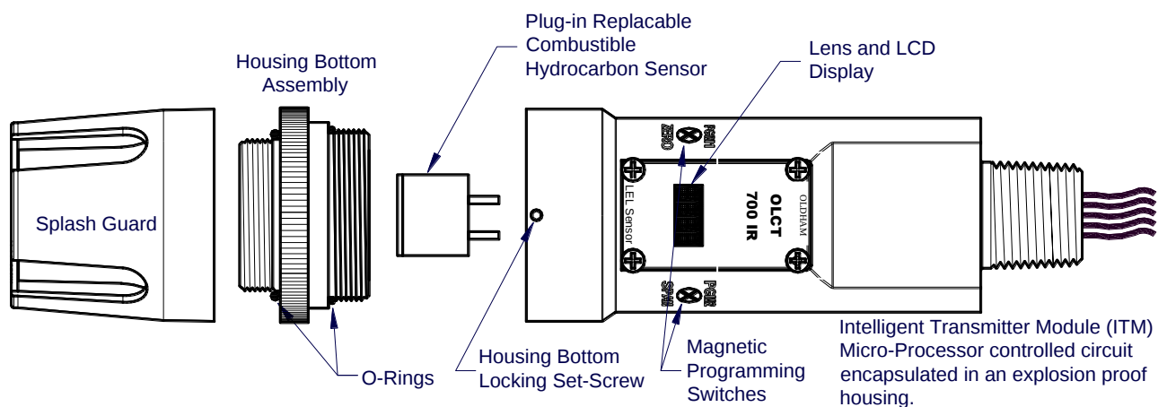
Figure 14: OLCT 700 Assembly
