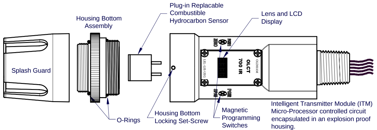
Figure 3: Detector Assembly Breakaway
