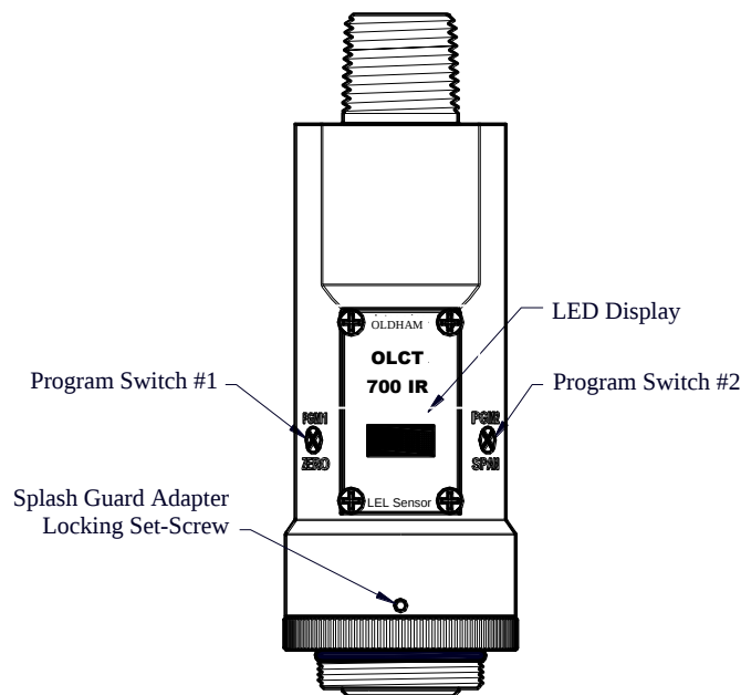
Figure 12: Magnetic Programming Switches
