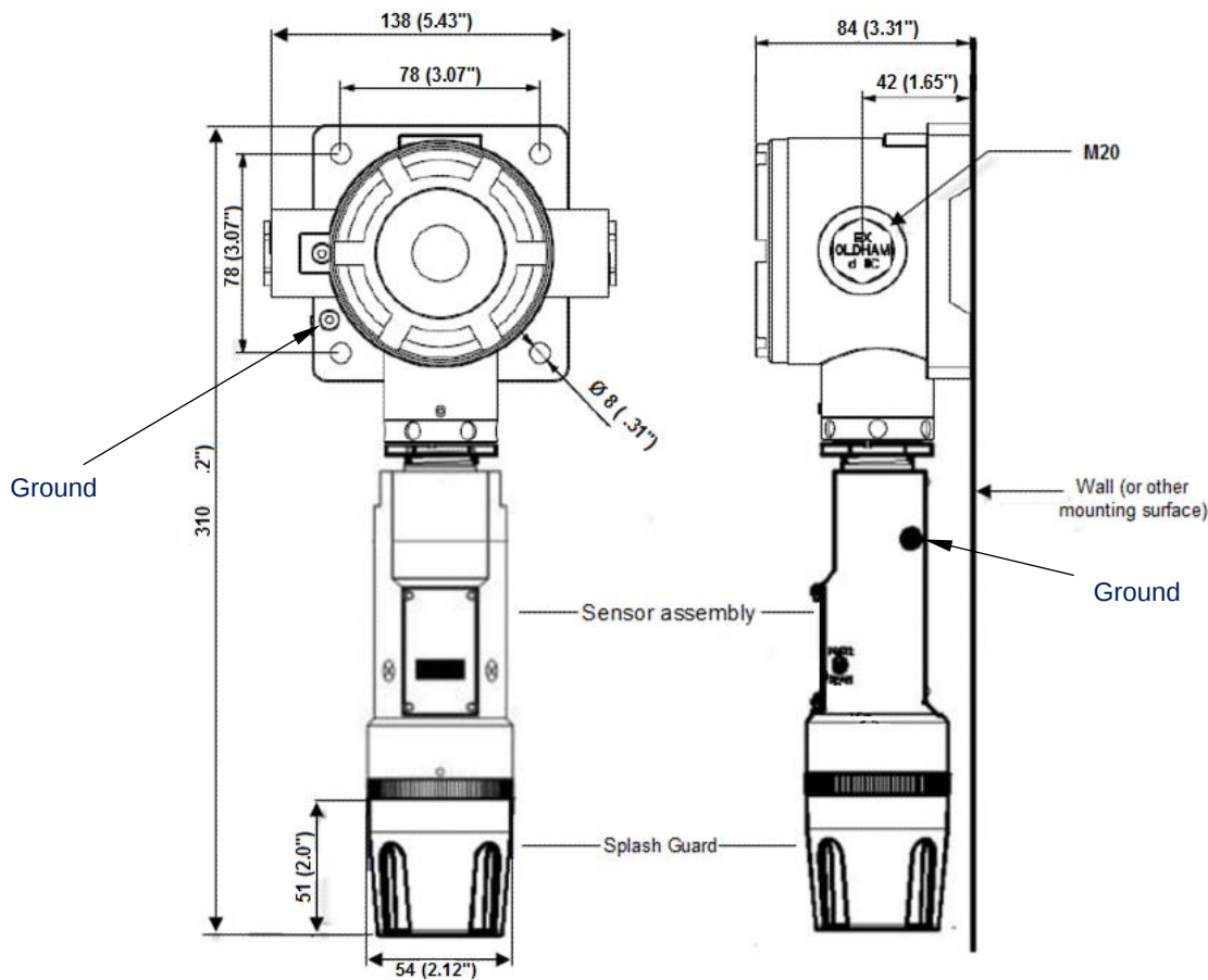
Figure 8: Outline and Mounting Dimensions
