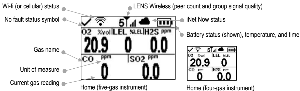
Figure 3.3 Power on
