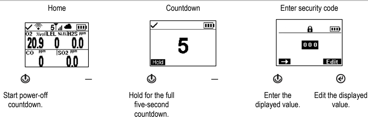
Figure 3.4 Power off
