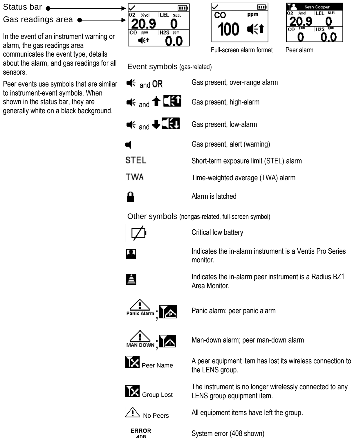
Figure 3.2.B Reading the display during an event (warning or alarm)
