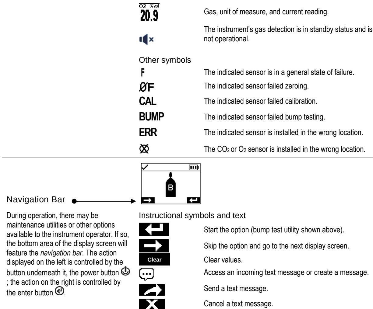
Figure 3.2.A Reading the display during operation
