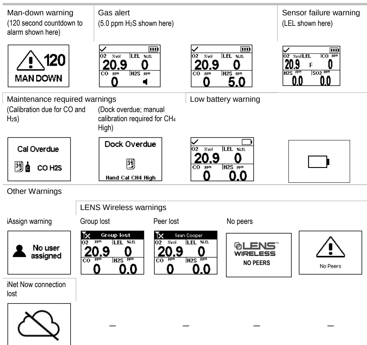
Figure 6.2 Warnings (display screens)
