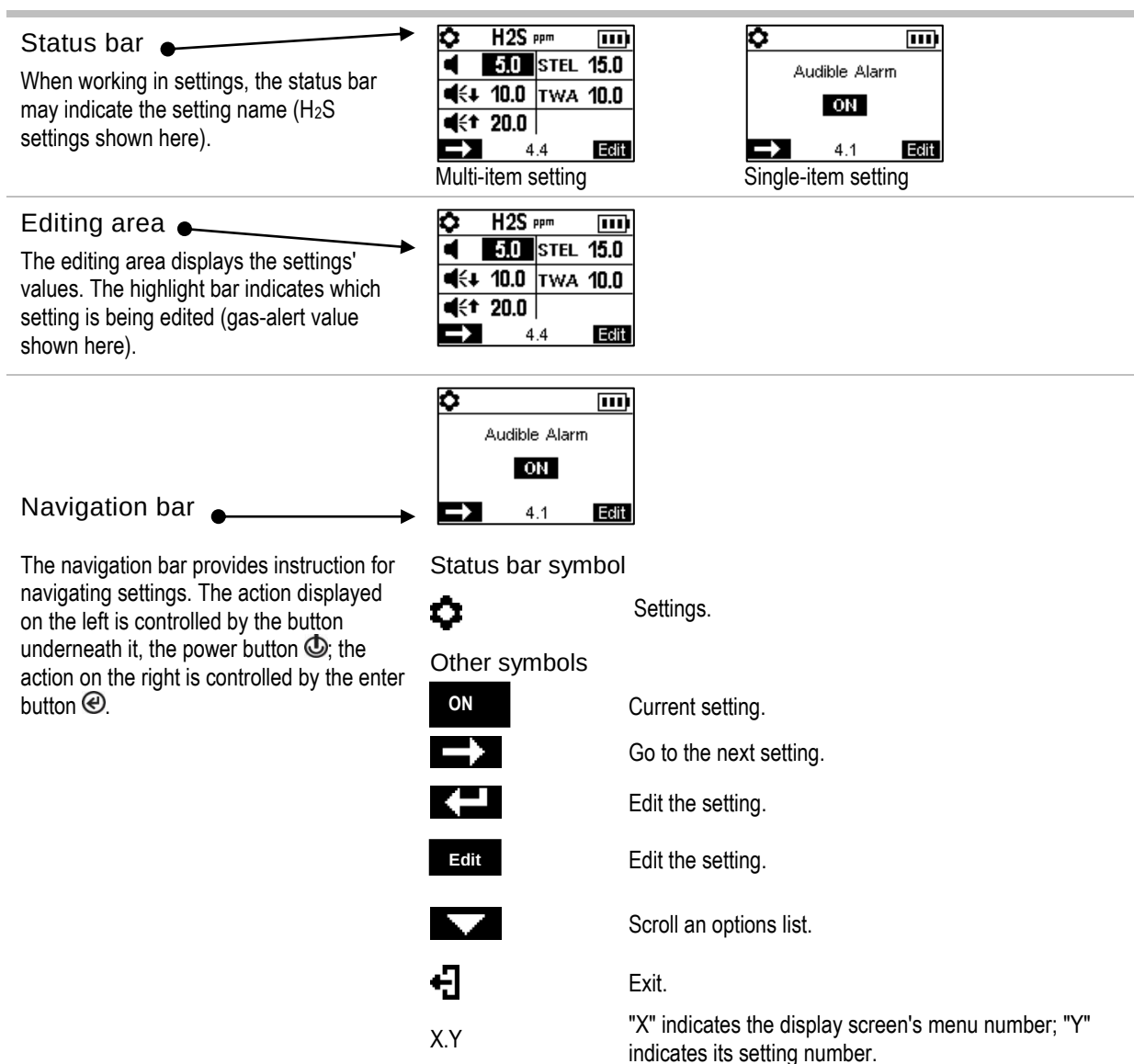
Figure 3.2.D Reading the display while working in settings
